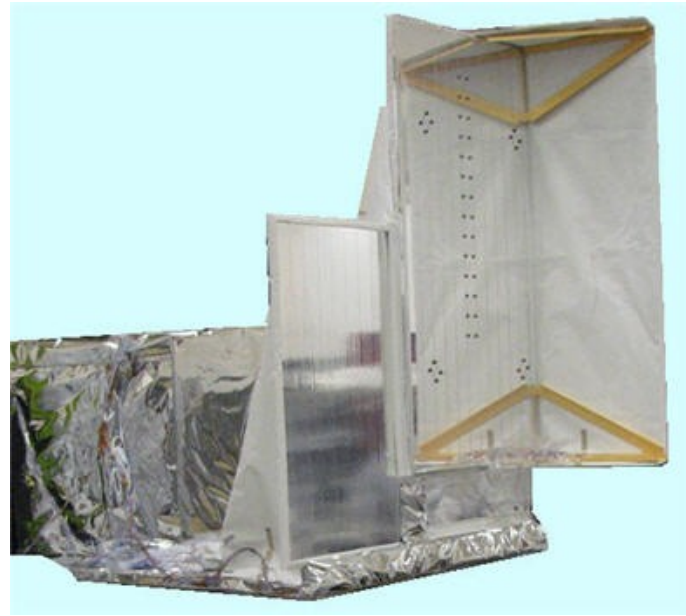
NASA LDCM Operational Land Imager Thermal Control Subsystem
