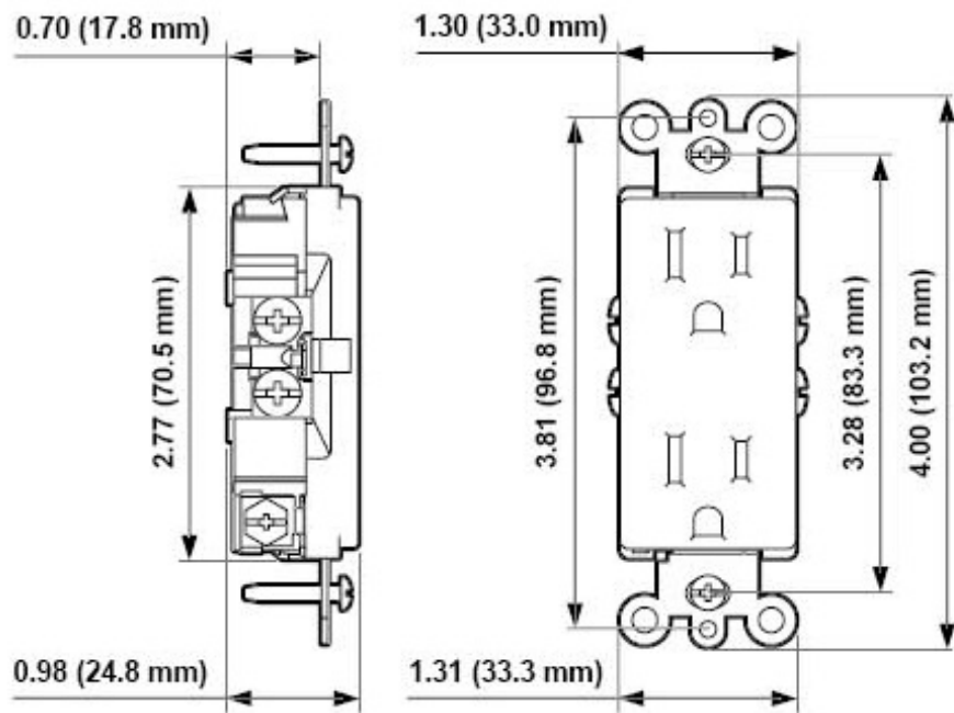
DUPLEX QUICKWIRE PUSH-IN AND SIDE-WIRED
